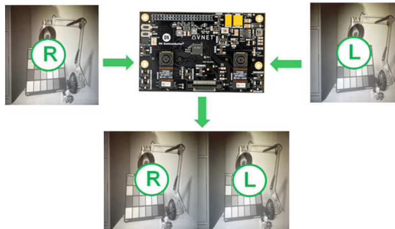
Figure 8.2: Dual AR0144 IAS Sensor Modules
